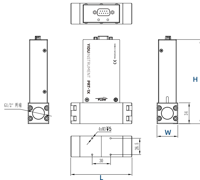
100SLPM~200SLPM 尺寸图
